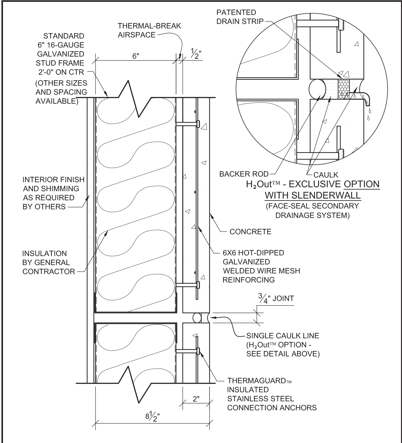
TYPICAL SLENDERWALL SECTION
